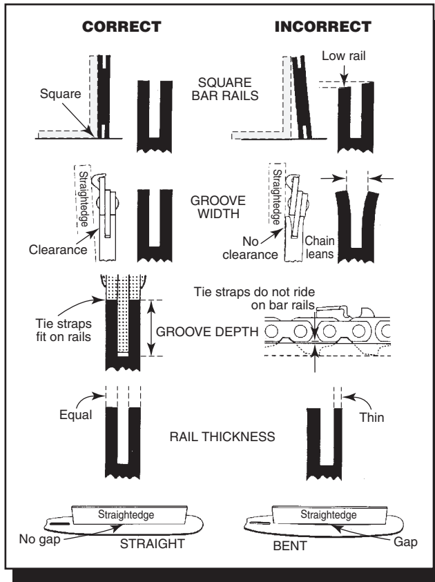
Figure 3-8—Correcting these rail conditions will prevent damage to the bar and cutting problems.—Oregon Maintenance and Safety Manual, permission by Blount, Inc.
