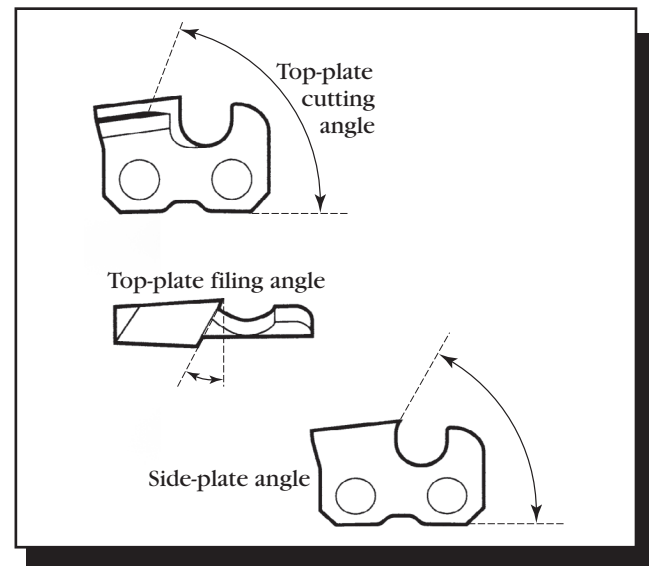
Figure 3-10—Maintain the top-plate cutting angle, top-plate filing angle, and side-plate angle.—Oregon Maintenance and Safety Manual, permission by Blount, Inc.
