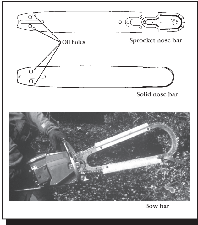
Figure 3-7—The three most common types of guide bars.—Oregon Maintenance and Safety Manual, permission by Blount, Inc.
