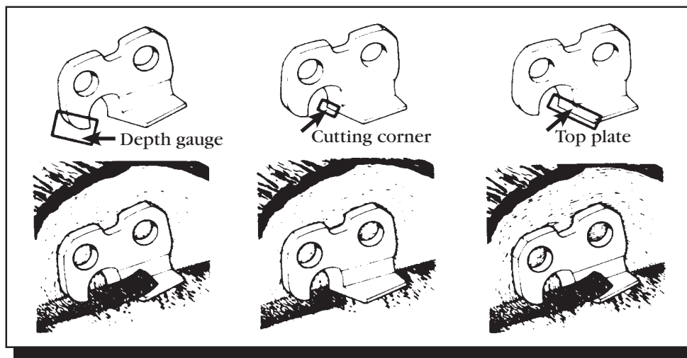
Figure 3-9—The depth gauge controls the depth at which a tooth's cutting corner bites into the wood.—Oregon Maintenance and Safety Manual, permission by Blount, Inc.
