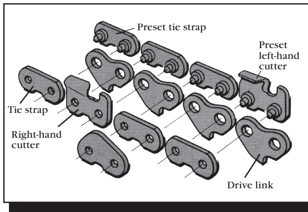
Figure 3-5—Parts of the chain.—Oregon Maintenance and Safety Manual, permission by Blount, Inc.
