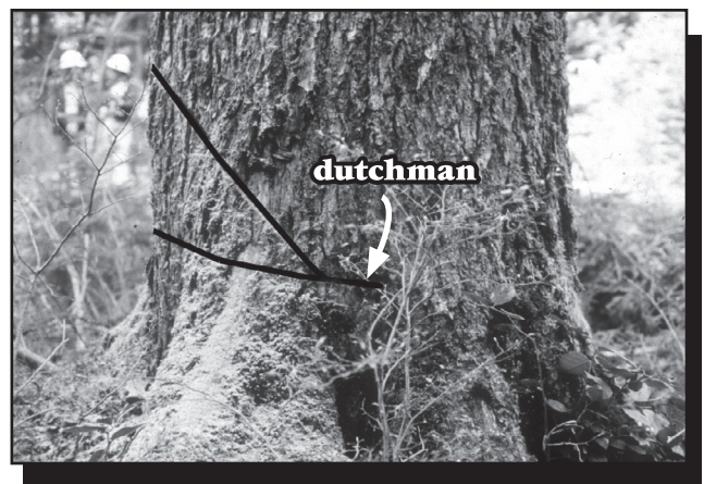
Figure 4-24—When the sloping cut and the horizontal cut do not meet exactly, a dutchman is formed. This kerf-wide cut makes the direction of the tree's fall harder to predict. It can also cause the tree to barber chair, lifting the log off the stump and placing the sawyer at great risk.
