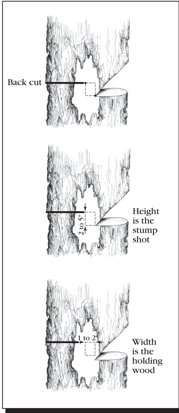
Figure 4-26—An imaginary rectangle can help the sawyer understand the importance of the back cut. The dimensions of this rectangle are based on a 24-inch-diameter tree.
