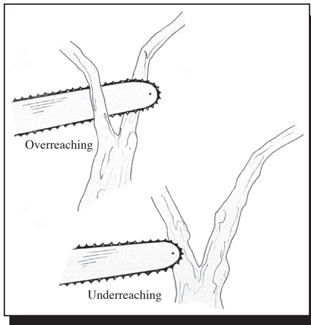
Figure 4-1—Avoid overreaching and underreaching kickbacks by using the bar properly.
