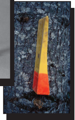
Figure 5-14—Triple-taper wedges allow a short wedge to provide as much lift as a longer wedge but require more force to drive.
