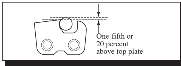
Figure 3-11—Hold the file at least one-fifth of the file's diameter above the cutter's top plate.—Oregon Maintenance and Safety Manual, permission by Blount, Inc.
