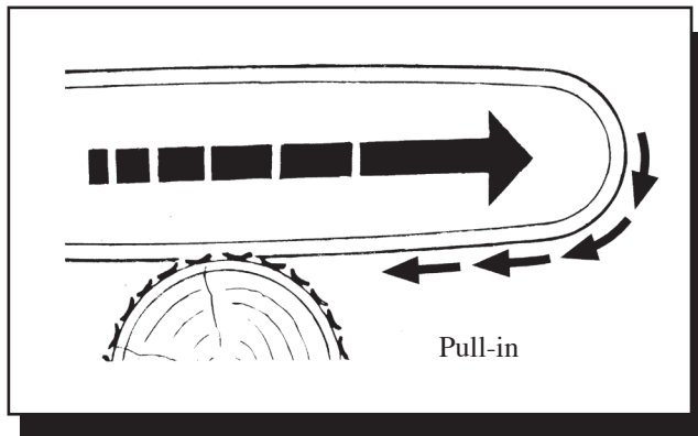
Figure 3-20—Pull-in occurs when the chain on the bottom of the bar is suddenly stopped by contacting another object or by being pinched.—From Chain Safety Manual, permission by Stihl, Inc.
