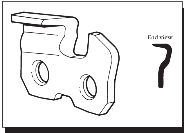
Figure 3-4—The semichisel cutter is less aggressive than the chisel cutter, will tolerate some dirt, and stays sharp longer than the chisel and the chipper cutters.—Oregon Maintenance and Safety Manual, permission by Blount, Inc.
