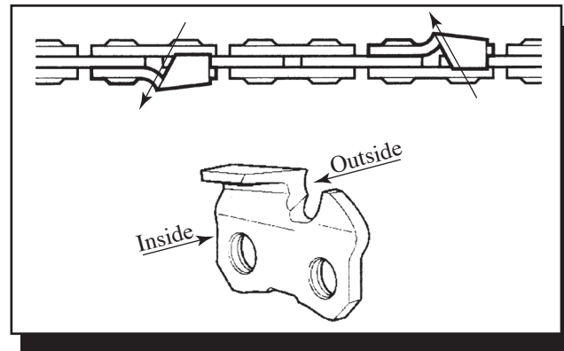
Figure 3-13—Sharpen the cutters on one side of the chain before turning the saw around to sharpen the other side.—Oregon Maintenance and Safety Manual, permission by Blount, Inc.
