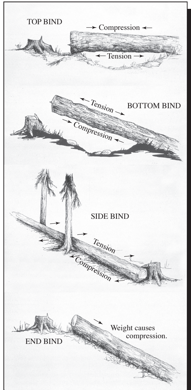
Figure 4-7—There are four types of binds. A log can have a combination of two or more binds.
